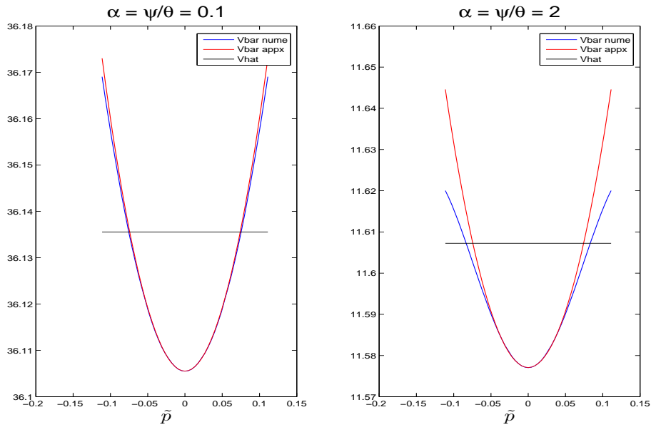
Figure AA-9: Numerical and approximated \bar{V} as a function of \alpha \equiv \frac{\psi}{\theta}
