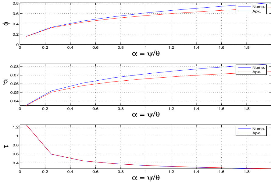
Figure AA-8: Numerical and approximated \phi , \tau, \bar{p} as a function of \alpha \equiv \frac{\psi}{\theta}
