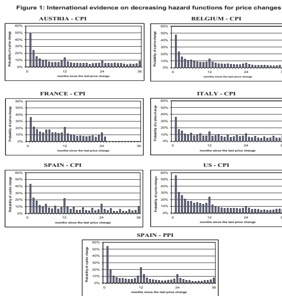
Figure AA-17: Hazard rate in Alvarez et al. (2005)
